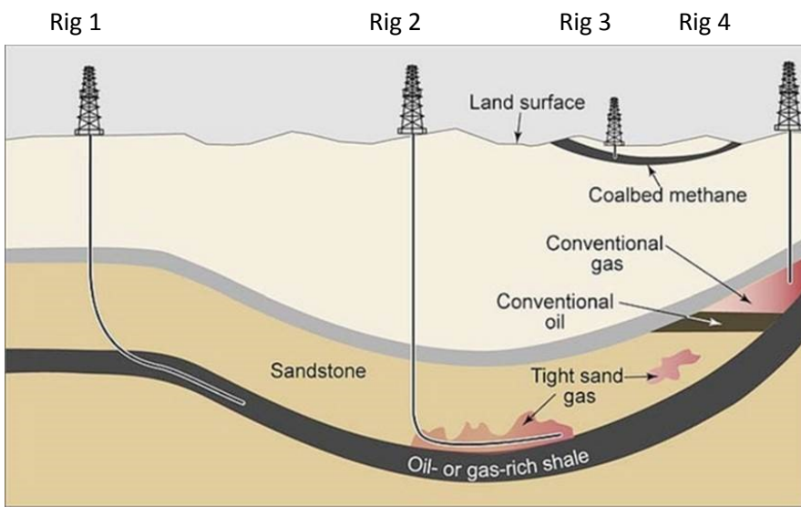
Cross Section of Shale Bed
